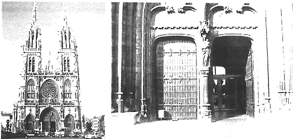
Figure 2: Gravity observations at Oostende station
